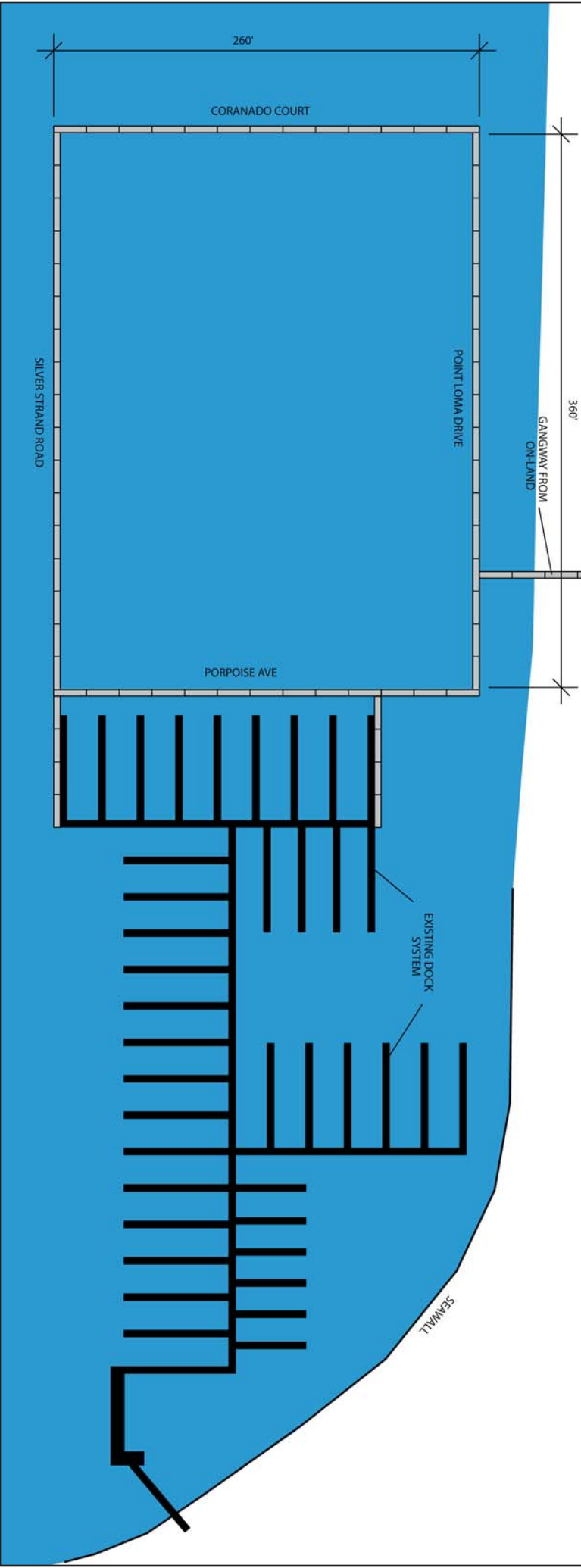
IN-WATER FLOOR PLAN -- SHERATON HOTEL/MARINA, HARBOR ISLAND
